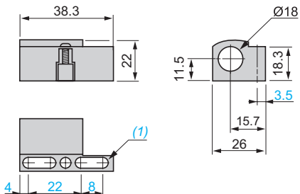
(1) 2 elongated holes Ø 4 X 8 mm
